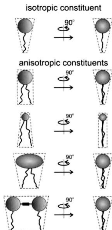
Fig. 1. Schematic representation of different intrinsic shapes of some membrane constituents. Front and side views are shown. Upper: isotropic constituent ( C_{1m} = C_{2m} ), lower: examples of anisotropic constituents ( C_{1m} \neq C_{2m} ).
