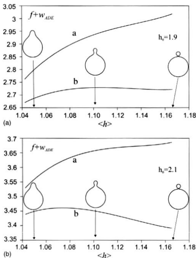
Fig. 7. Bilayer membrane free energy including non-local isotropic bending as a function of the average mean curvature of the vesicle with \nu = 0.95 and q = 2 . Curves a: local and non-local isotropic bending ( \beta = 0 , \kappa = 0 ). Curves b: local and non-local isotropic bending and deviatoric bending due to the orientational ordering ( \beta = 1.5 \times 10^{-4} , \kappa = 7 \times 10^6 ).
