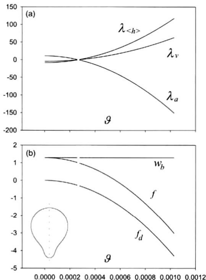
Fig. 2. (a) Lagrange coefficients as a function of the interaction constant g . (b) Bilayer membrane free energy f and the energy contributions: energy of isotropic bending w_b , and contribution of orientational ordering f_d as a function of the interaction constant g . The values of model parameters are \nu = 0.95 , \langle h \rangle = 1.0422 , \kappa = 7 \times 10^6 (from Kralj-Iglic et al [14]).
