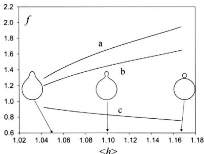
Fig. 6. Bilayer membrane free energy as a function of the average mean curvature of the vesicle with v = 0.95 ; (a) isotropic bending, (b) orientational ordering of independent molecules \beta = 1.5 \times 10^{-4} , \kappa = 7 \times 10^6 , c: orientational ordering of interacting molecules \beta = 3 \times 10^{-4} , \kappa = 7 \times 10^6 (adapted from [14]).
