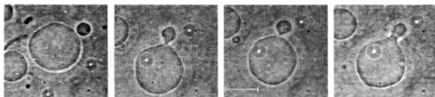
Fig. 5. Oscillations of the neck width before the neck opens and the vesicle attains its flaccid shape indicating that the shape with the narrow neck is energetically favorable, bar = 20 \mu m (adapted from Iglic and Kralj-Iglic [17]).
