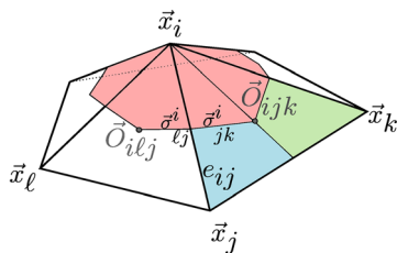
Fig. 16 Schematic of a vertex and its neighbors. The vertex i has neighbors, \ell, j, k, \dots , which are connected by edges e_{j\ell}, \dots , where we explicitly show e_{ij} . Each triangle has a circumcenter O , and the area is assigned to each of the 3 vertices, which is shown for triangle ijk (red, green, and blue section). The total area assigned to i is shown in red across the entire cap, and the dual edge \sigma^i across e_{ij} are shown \sigma^i_{jk} and \sigma^i_{j\ell} . The curvature of vertex i is essentially computed on the red area, for example, the normal of the vertex N(i) is the average of the local normal for every point in the red surface.
