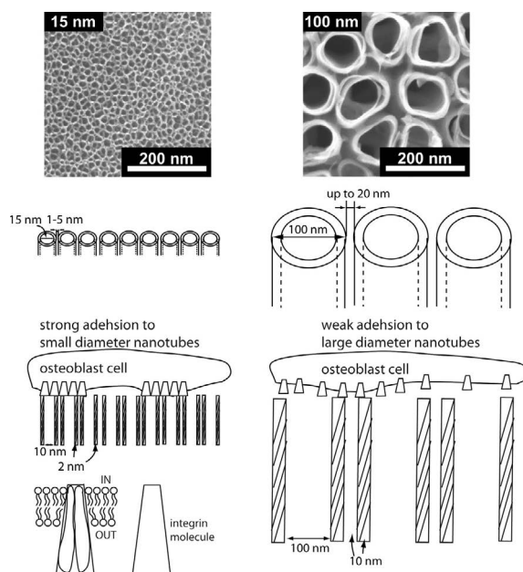
Figure 14.25 Hypothetical model explaining the observed differences in the binding strength of small and large diameter \text{TiO}_2 nanotubes. Electron microscope images of surfaces of vertically aligned \text{TiO}_2 nanotubes. Note that the small diameter (15 nm) nanotubes are much more closely packed than the large diameter (100 nm) \text{TiO}_2 nanotubes. The inner and outer diameter of a small diameter nanotube are approximately 10 nm and 15 nm, and the respective dimensions of a large diameter nanotube are approximately 80 nm and 100 nm. The small diameter nanotube surface has a significantly larger proportion of strong integrin binding regions (due to the larger area density of highly curved nanotube edges) than the large diameter nanotube surface. In addition, the extracellular part of the integrin molecules (of conical shapes) could bind to neighbouring nanotubes on the small diameter nanotube surface, which is not possible on a nanotube surface having too large a hollow interior space, since the interacting integrin molecules are in contact with the nanotube edges. Reprinted from Gongadze, E., Kabaso, D., Bauer, S., Park, J., Schmuki, P., and Igljč, A. (2012). Adhesion of Osteoblast to a Vertically Aligned \text{TiO}_2 Nanotube Surface. Mini-Reviews in Medicinal Chemistry . 13, 194–200, by permission of Eureka Science Ltd., copyright 2012, and republished with permission of DOVE Medical Press, from Gongadze, E., Kabaso, D., Bauer, S., Slivnik, T., Schmuki, P., van Rienen, U., and Igljč, A. (2011). Adhesion of osteoblasts to a nanorough titanium implant surface. Int. J. Nanomed. , 6, pp. 1801–1816.; permission conveyed through Copyright Clearance Center, Inc.
