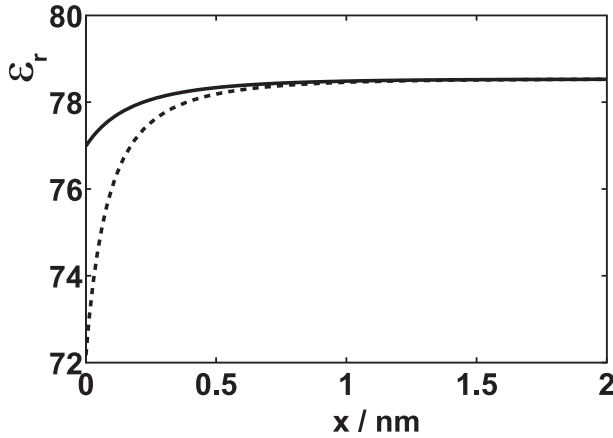
Figure 13.8 Relative dielectric permittivity \varepsilon_r as a function of the distance from the charged surface x within the presented Langevin PB theory for point-like ions. Equations 13.91–13.95 were solved numerically using the finite element method (FEM) within the program package Comsol Multiphysics Software as described in (Gongadze et al., 2011c). Dipole moment of water p_0 = 4.79 D, bulk concentration of salt n_0/N_A = 0.15 mol/l, bulk concentration of water n_{0w}/N_A = 55 mol/l, surface charge density \sigma = -0.1 A s/m 2 (full line) and \sigma = -0.2 A s/m 2 (dashed line).
