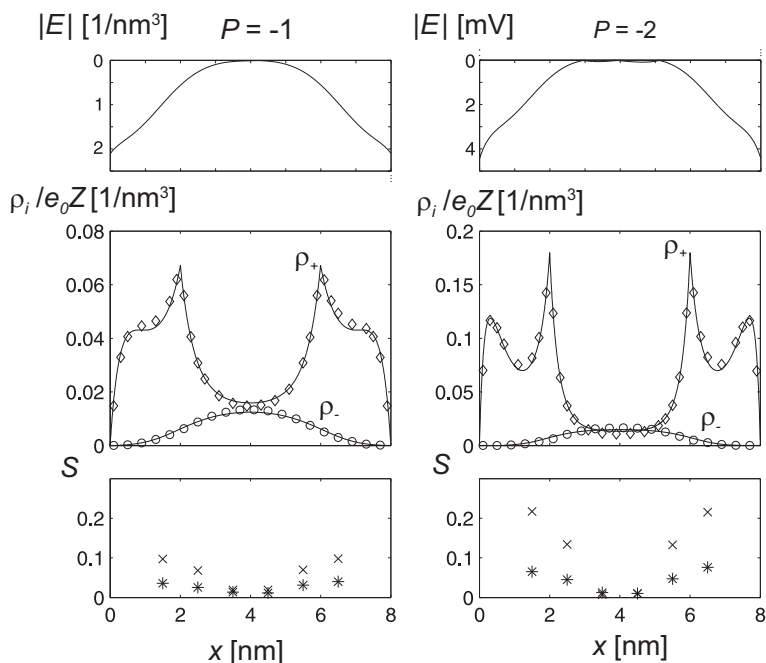
Figure 14.13 The spatial dependence of the magnitude of electric field strength (first row), the volume charge density of the positively charged nanoparticles (counterions) and negatively charged nanoparticles (coions) (second row), and the average order parameter S computed in six slices along the x -axis (positive nanoparticles: crosses, negative nanoparticles: stars) (third row) in the space between the two charged surfaces at the distance D = 8 nm. The value of the charge parameter: P = -1 (first column), P = -2 (second column). The values of other model parameters: l = 2 nm, Z = 1 . Reprinted with kind permission from Springer Science+Business Media: Perutková, Š., Frank, M., Bohinc, K., Bobojevič, K., Zelko, J., Rozman, B., Kralj-Iglič, V., and Iglič, A. (2010). Interaction between equally charged membrane surfaces mediated by positively and negatively charged nanoparticles. J. Membr. Biol. , 236, pp. 43–53.
