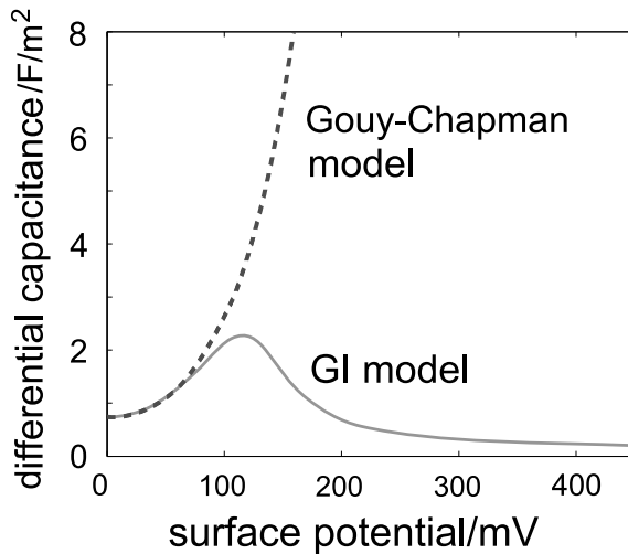
Figure 13.12 Differential capacitance as a function of the surface potential using Gouy–Chapman Eq. 13.137 (dashed line) and numerically by using GI Eq. 13.122 (full line). Figure adapted from Gongadze et al. (2013).
