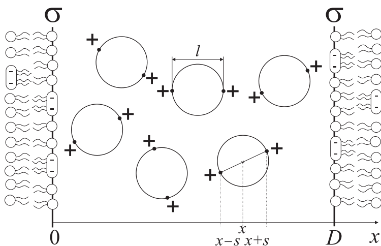
Figure 14.5 Schematic illustration of two negatively charged planar surfaces with surface charge density \sigma separated by a solution containing spherical charged nanoparticles (counterions) with spatially distributed positive charge. The charges within a counterion are separated by a fixed distance l = a , where a is the diameter of the nanoparticles. Reprinted with kind permission from Springer Science+Business Media: Perutková, Š., Frank, M., Bohinc, K., Bobojevič, K., Zelko, J., Rozman, B., Kralj-Iglič, V., and Iglič, A. (2010). Interaction between equally charged membrane surfaces mediated by positively and negatively charged nanoparticles. J. Membr. Biol. , 236, pp. 43–53.
