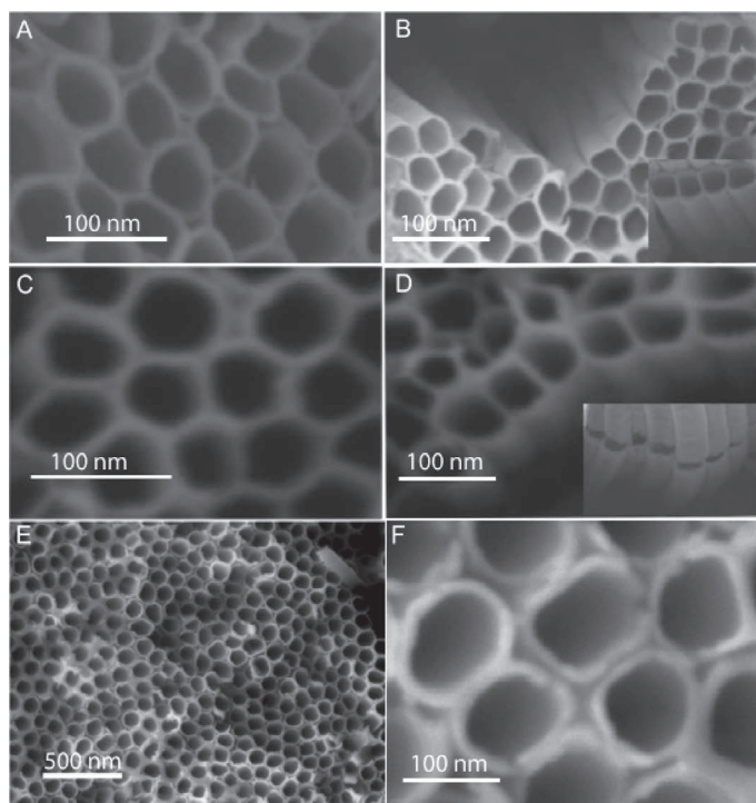
Figure 14.20 Electron microscope images of surface layers of self-assembled vertically aligned \text{TiO}_2 nanotubes synthesized by the anodization method. For preparation, an ethylene glycol solution with 0.3 wt. was used. The internal \text{TiO}_2 nanotube diameter is around 50–60 nm (A–D) and 100 nm (E–F), while the length could be up to 10 \mu\text{m} (B) Reprinted from Imani, R., Kabaso, D., Kreft, M. E., Gongadze, E., Penič, S., Elersič, K., Kos, A., Vršanič, P., Zorec, R., and Iglič, A. Morphological alterations of T24 cells on flat end nanotubular \text{TiO}_2 surfaces. Croat Med. J. , 53, pp. 577–585. Copyright © 2012 by the Croatian Medical Journal. All rights reserved.
