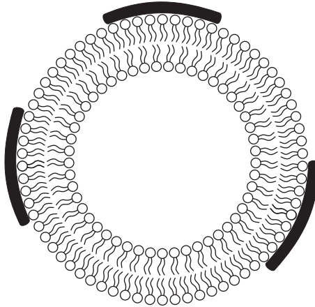
Figure 12.3 Schematic figure of the cross-section of a bilayer membrane tubular protrusion with attached FRPs having C_p > 0 . The rotation angle \omega = 0 .
