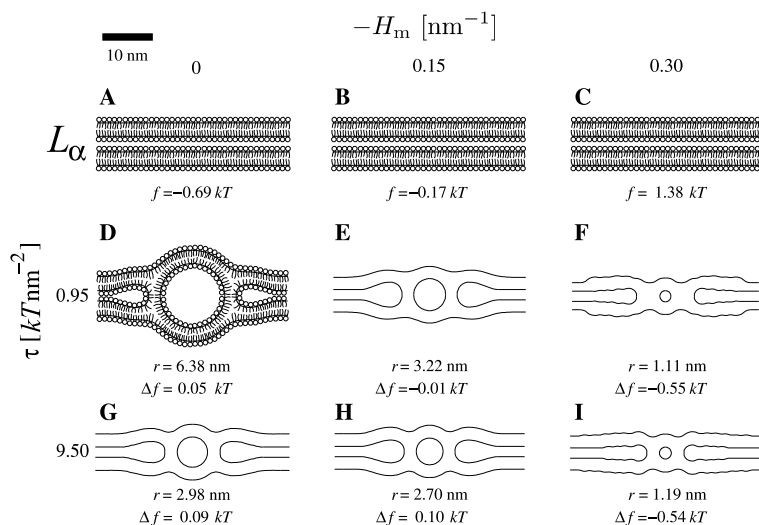
Figure 7.12 Configuration of a system of two monolayers, a cylinder of H_{II} phase and two bulb-like closures representing a nucleation line in the L_{\alpha} - H_{II} transition for different intrinsic curvatures H_m and different stretching moduli of the phospholipid chains \tau . We assume that phospholipid molecules are anisotropic corresponding to D_m = |H_m| . The free energy per lipid molecule and the radius of the central cylinder are given for each configuration. Reprinted with permission from Mareš, T., Daniel, M., Perutkova, Š., Perne, A., Dolinar, G., Iglič, A., Rappolt, M., and Kralj-Iglič, V. Role of phospholipid asymmetry in the stability of inverted hexagonal mesoscopic phases. J. Phys. Chem. B , 112(51), pp. 16575–16584. Copyright 2008, American Chemical Society.
