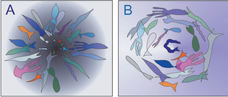
Figure 1.1 Schematic figure of a source of a vector field (a) and a vortex of the vector field (b).
