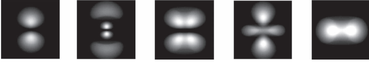
Figure 1.6 Schematic figure of the probability density of an electron in the hydrogen atom. Different probability densities correspond to different eigenstates. Lighter areas mean larger probability densities (image: http://blazelabs.com ).
