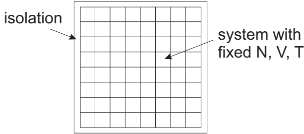
Figure 1.7 Scheme of a canonical ensemble, composed of \mathcal{M} systems. Each system has volume V and N constituents. The temperature in all the systems is T . The ensemble, isolated with respect to the surroundings, is considered as a supersystem with volume \mathcal{M}V , number of constituents \mathcal{M}N , and energy E_t .
