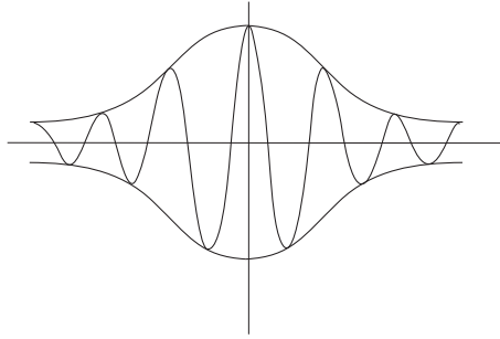
Figure 1.5 A wave packet.
