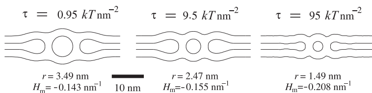
Figure 7.13 Nucleation configurations for different values of the stretching modulus of phospholipid tails ( \tau ) at the transition point from L_\alpha to H_{II} phase where \Delta f = 0 . Anisotropic case ( D_m = |H_m| ). Reprinted with permission from Mareš, T., Daniel, M., Perutková, Š., Perne, A., Dolinar, G., Iglič, A., Rappolt, M., and Kralj-Iglič, V. Role of phospholipid asymmetry in the stability of inverted hexagonal mesoscopic phases. J. Phys. Chem. B. , 112(51), pp. 16575–16584. Copyright 2008, American Chemical Society.
