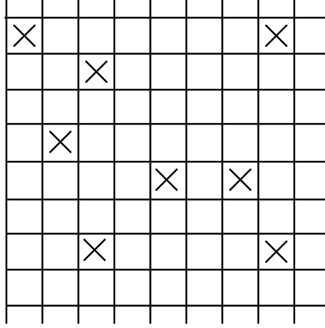
Figure 13.2 Schematic representation of the lattice model, where only counterions are included.
