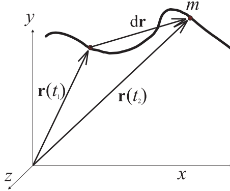
Figure 1.3 Within classical mechanics the motion of a point-like particle with mass m in three dimensional space (x, y, z) is described by time-dependent (t) radius (position) vector \mathbf{r}(t) . Here t_1 < t_2 .
