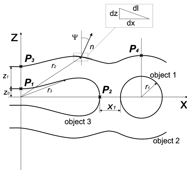
Figure 7.11 Parametrization of the pivotal surface. A bulb-like closure (object 3) is placed between adjacent bilayers (objects 2) is a cylinder (object 1). The geometry of the system is symmetrical with respect to the x -axis. Reprinted with permission from Mareš, T., Daniel, M., Perutková, Š., Perne, A., Dolinar, G., Iglič, A., Rappolt, M., and Kralj-Iglič, V. Role of phospholipid asymmetry in the stability of inverted hexagonal mesoscopic phases. J. Phys. Chem. B. , 112, 51, pp. 16575–16584. doi: 10.1021/jp805715r. Copyright 2008 American Chemical Society.
