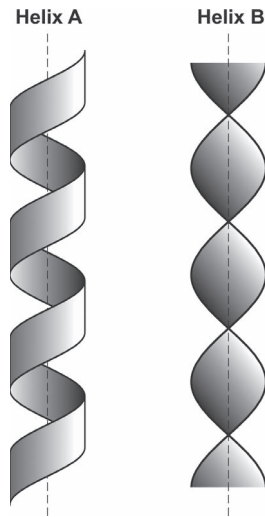
Figure 8.4 Schematic representation of helical configurations A and B.
