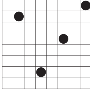
Figure 1.8 Two dimensional representation of a lattice with M = 64 sites and N = 4 system constituents.
