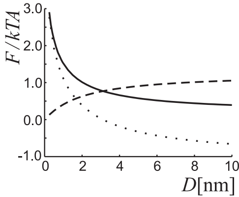
Figure 14.3 Free energy (full line), electrostatic energy (dashed line), and configurational entropy (dotted line) as a function of the distance between the equally charged surfaces D . Parameters of PB equation and corresponding free energy expression are: |\sigma| = 0.1 \text{ As/m}^2 and v_0 = 5 \text{ nm}^3 .
