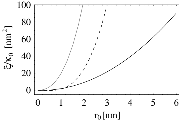
Figure 8.10 Interaction constant \xi (Eq. 8.22) as a function of the average radius of the rigid protein ( r_0 ) in the model of constrained local membrane microscopic shape perturbations (Fig. 8.5A) calculated from Eq. 8.27 for \zeta = 0.9 nm (grey full curve) and from Eq. 8.47 (dashed curve) for \eta^2 = 1 , \bar{\alpha} = -0.2 and \tilde{\zeta}_c = 0.2 nm. The figure also shows the dependence of \xi on r_0 for unconstrained local membrane microscopic shape perturbations (Fig. 8.5B), as calculated from Eqs. 8.46 for \tilde{\zeta} = 0.2 nm and same values of \eta^2 and \bar{\alpha} (black solid curve).
