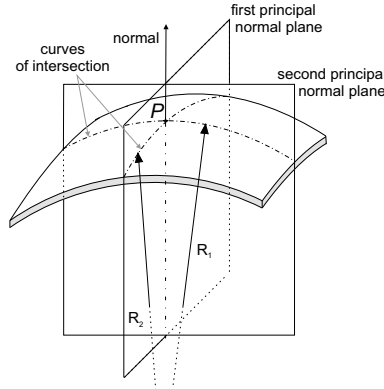
Figure 5.1 A schematic figure of the two principal normal planes and the corresponding two principal curvature radii R_1 and R_2 , which define the two principal curvatures C_1 = 1/R_1 and C_2 = 1/R_2 . Figure adapted from Perutková et al. (2009).
