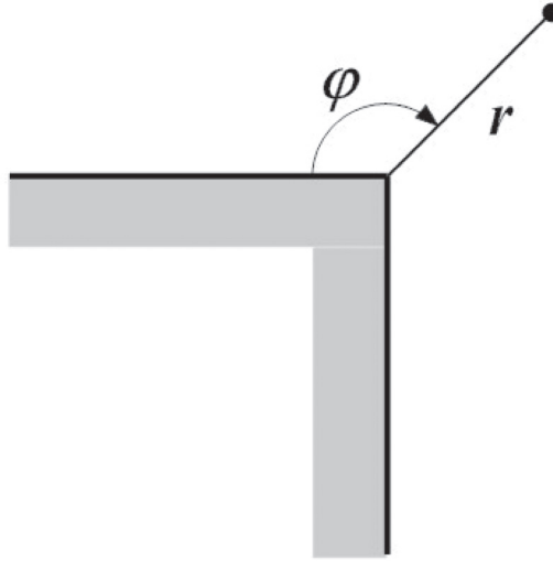
Figure 14.23 Schematic figure of the convex edge of the implant surface in the limit of very high curvature.
