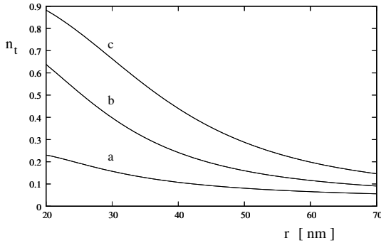
Figure 9.2 Fraction of the area of membrane tubular protrusions covered by anisotropic nanodomains ( n_t ) as a function of the curvature radius of the tube ( r ) for three values of the intrinsic curvature deviator of the nanodomains (inclusions) ( D_m ): 0.03 \text{ nm}^{-1} (a), 0.04 \text{ nm}^{-1} (b) and 0.05 \text{ nm}^{-1} (c). The values of the other model parameters are: \bar{n} = 0.02 , a_2 = 0.02 , H_m = D_m , w/kT = 0.125 and \xi = 5000 \text{ kT nm}^2 . Reprinted from Journal of Theoretical Biology , 240(3), Aleš Iglič, Henry Hägerstrand, Peter Veranič, Ana Plemenitaš, and Veronika Kralj-Iglič, Curvature-induced accumulation of anisotropic membrane components and raft formation in cylindrical membrane protrusions, pp. 368–373, Copyright 2006, with permission from Elsevier.
