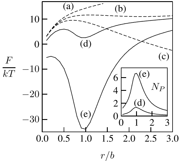
Figure 16.2 The pore free energy, F , as a function of the pore size r . The dashed lines correspond to a charged inclusion-free membrane of charge density \sigma = -0.05 \text{ As/m}^2 with Debye length l_D = 2.6 \text{ nm} (a), l_D = 2.8 \text{ nm} (b), and l_D = 3.0 \text{ nm} (c). The solid lines describe the effect of adding anisotropic inclusions (characterized by K_1 = 98 kT \text{ nm}^2 , K_2 = -65 kT \text{ nm}^2 , C_{1m} = -C_{2m} = 1/b ) to the charged membrane with \sigma = -0.1 \text{ As/m}^2 and l_D = 2.8 \text{ nm} . The average area density of inclusions n is 1/70000 \text{ nm}^2 (d) and 1/14000 \text{ nm}^2 (e). The inset shows the corresponding numbers, N_P , of inclusions within the membrane rim for curves (d) and (e). Reprinted with permission from Fošnarič, M., Kralj-Iglič, V., Bohinc, K., Iglič, A., and May, S. Stabilization of pores in lipid bilayers by anisotropic inclusions. J. Phys. Chem. B , 107, pp. 12519–12526. Copyright 2003, American Chemical Society.
