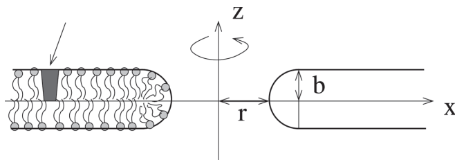
Figure 16.1 A planar lipid bilayer with a pore of radius r in the centre. The figure shows the cross-section in the x - z plane. Rotational symmetry around the z -axis is indicated. On the left side, the packing of lipid molecules is shown schematically. The head-groups of lipid molecules are represented by circles. The arrow denotes a membrane inclusion (single molecule or nanodomain) which is shown schematically. The local geometry within the rim is saddle-like everywhere. The semi-toroidal shape of the pore rim is an assumption; alternative pore shapes could be considered, but are not expected to alter the main conclusions of the theoretical analysis. Reprinted with permission from Fošnarič, M., Kralj-Iglič, V., Bohinc, K., Iglič, A., and May, S. Stabilization of pores in lipid bilayers by anisotropic inclusions. J. Phys. Chem. B , 107, pp. 12519–12526. Copyright 2003, American Chemical Society.
