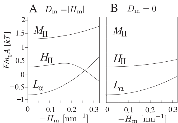
Figure 7.4 The equilibrium free energy per lipid molecule F/n_0 A = F_b/n_0 A + F_i/n_0 A consisting of the contribution of bending ( F_b ) and (constant) void-filling energy ( F_i ), calculated per lipid molecule as a function of the intrinsic mean curvature |H_m| for the L_\alpha ( F_i/n_0 A = 0 ), H_{II} ( F_i/n_0 A = 1kT ) and M_{II} ( F_i/n_0 A = 2kT ) phases. A: D_m = |H_m| and B: D_m = 0 , \tilde{k}/kT = 1 . Reprinted with permission from Mareš, T., Daniel, M., Perutková, Š., Perne, A., Dolinar, G., Iglič, A., Rappolt, M., and Kralj-Iglič, V. Role of phospholipid asymmetry in the stability of inverted hexagonal mesoscopic phases. J. Phys. Chem. B , 112(51), pp. 16575–16584. Copyright 2008, American Chemical Society.
