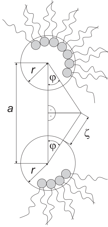
Figure 7.8 Scheme of two neighbouring inverted lipid tubes in a hexagonal lattice. The lipid tails have to stretch in order to fill voids in the hydrocarbon region. The symbol a denotes the H_{II} phase lattice constant and r denotes the radius of the pivotal plane of the H_{II} phase. The actual length of hydrocarbon tails ( \zeta ) depends on the angle \varphi (Perutková et al., 2009).
