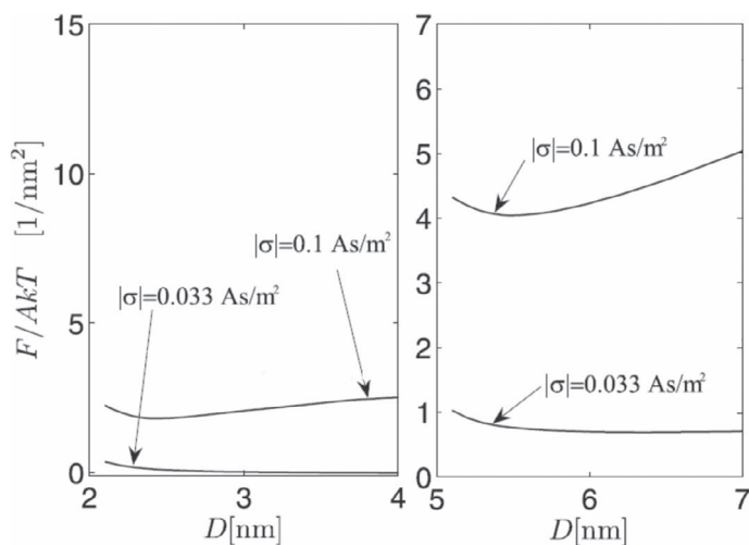
Figure 14.6 Normalized free energy f (Eq. 14.7) as a function of the distance between the negatively charged surfaces D for Z = 1 , two different surface charge densities: \sigma = -0.033 As/m 2 and \sigma = -0.1 As/m 2 , and two different distances between the charges within the nanoparticle: l = 2 nm (left left), l = 5 nm (right figure), l_B = 0.7 nm. Reprinted with permission from Urbanija, J., Bohinc, K., Bellen, A., Maset, S., Iglič, A., Kralj-Iglič, V., and Sunil Kumar, P. B. (2008b). Attraction between negatively charged surfaces mediated by spherical counterions with quadrupolar charge distribution. J. Chem. Phys. , 129, pp. 105101. Copyright 2008, AIP Publishing LLC.
