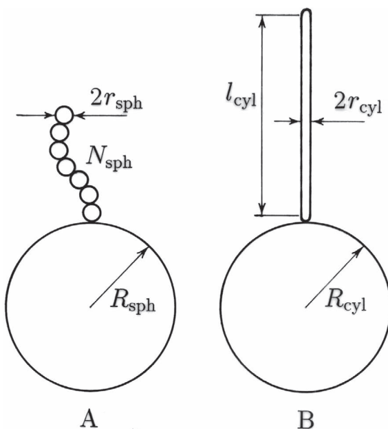
Figure 7.14 Schematic representation of a shape composed of the mother sphere and a protrusion composed of small spheres connected by infinitesimal necks (A), and of a shape composed of the mother sphere and a thin cylinder closed by hemispherical caps (B).
