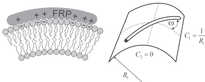
Figure 12.1 Schematic figure of a flexible rod-like protein (FRP) strongly attached to a cylindrical membrane surface having C_1 = 1/R_1 and C_2 = 0 , that is, H = D = 1/2 R_1 . At a given value of the protein orientation angle \omega , the protein senses the curvature C = (C_1 + C_2)/2 + [(C_1 - C_2)/2] \cos(2\omega) . Reprinted from Journal of Biomechanics , 43(8), Šarká Perutková, Veronika Kralj-Iglič, Mojka Frank, and Aleš Iglič, Membrane stability of membrane nanotubular protrusions influenced by attachment of flexible rod-like proteins, pp. 1612–1617, Copyright 2010, with permission from Elsevier.
