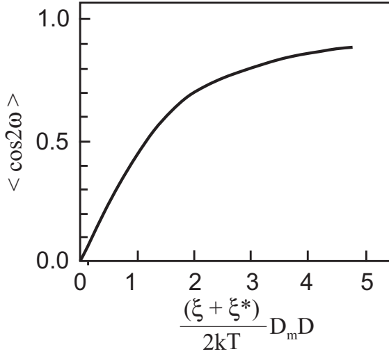
Figure 7.2 Average orientation of a single lipid molecule described by \langle \cos(2\omega) \rangle as a function of (\xi + \xi^*)DD_m / 2kT (see Iglič et al., 2000).
