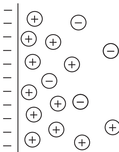
Figure 13.1 Schematic representation of a planar EDL composed of a negatively charged planar surface in contact with an electrolyte solution of positively charged counterions and negatively charged coions. The counterions accumulate near the charged surface.
