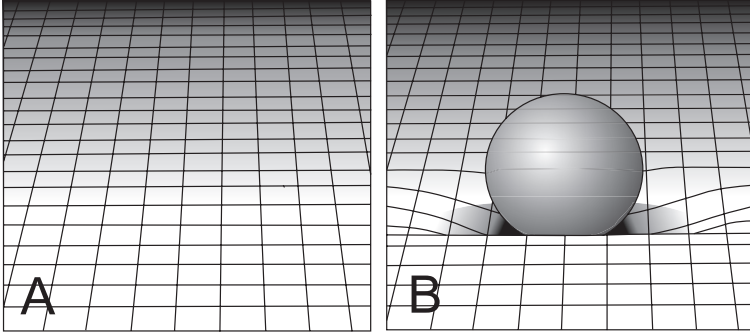
Figure 1.4 A two-dimensional representation of flat space (A). Due to the presence of mass (a sphere), space is curved (B).
