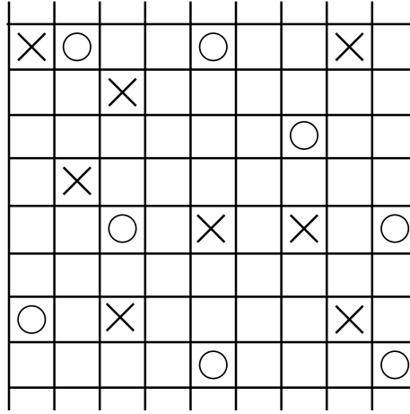
Figure 13.3 Schematic representation of the lattice model in which counterions ( \times ) and coions ( \circ ) are included.
