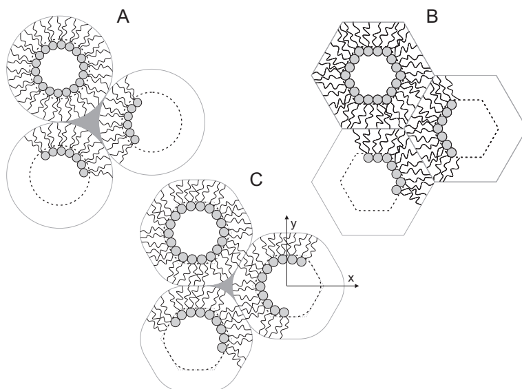
Figure 7.7 Schemes of the approaches by different authors to the geometry of the inverted hexagonal phase: (A) a circular cross-section (Rand et al., 1990; Siegel, 1993), (B) hexagonal cross section (Hamm and Kozlov, 1998), (C) intermediate between circular and hexagonal cross section (Malinin and Lentz, 2004; Perutková et al., 2009).
