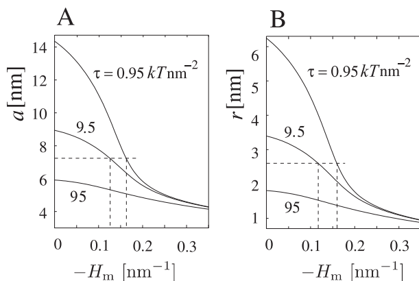
Figure 7.10 Structural parameters of the H II phase for inverted wedge-like shaped lipids with D_m = |H_m| (see Figs. 6.1D and 7.5). The optimal unit cell parameter a (A) and the optimal pivotal plane radius r (B) are plotted versus the absolute value of the mean curvature H_m for different lipid chain rigidities \tau and \tilde{k}/kT = 1 . The two horizontal dashed lines mark realistic values for a and r , respectively (Table 7.1). For definitions of a and r see Fig. 6.4. Reprinted with permission from Mareš, T., Daniel, M., Perutkova, Š., Perne, A., Dolinar, G., Iglič, A., Rappolt, M., and Kralj-Iglič, V. Role of phospholipid asymmetry in the stability of inverted hexagonal mesoscopic phases. J. Phys. Chem. B , 112(51), pp. 16575–16584. Copyright 2008, American Chemical Society.
