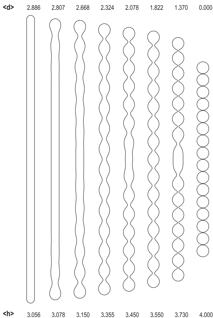
Figure 9.9 A series of prolate vesicle shapes calculated by minimization of the local membrane bending energy (Eq. 7.30) as described in (Iglič et al., 1999). The relative volume v = 1/\sqrt{16} (see also Section 7.8). The corresponding values of \langle h \rangle = R\langle H \rangle and \langle d \rangle = R\langle D \rangle are also given. Here R = \sqrt{A/4\pi} . Reprinted from Journal of Biomechanics , 43(8), Šarká Perutková, Veronika Kralj-Iglič, Mojka Frank, and Aleš Iglič, Membrane stability of membrane nanotubular protrusions influenced by attachment of flexible rod-like proteins, pp. 1612–1617, Copyright 2010, with permission from Elsevier.
