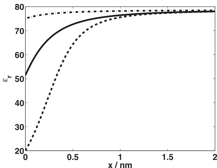
Figure 13.11 Relative permittivity \varepsilon_r (Eq. 13.121) as a function of distance from a planar charged surface x . Three values of surface charge density were considered: \sigma = -0.1 \text{ A s/m}^2 (dashed-dotted line), \sigma = -0.2 \text{ A s/m}^2 (full line) and \sigma = -0.3 \text{ A s/m}^2 (dashed line). Values of parameters assumed were dipole moment of water p_0 = 3.1 \text{ D} , bulk concentration of salt n_0/N_A = 0.15 \text{ mol/l} , n = 1.33 , n_{ow}/N_A = 55 \text{ mol/l} . Reprinted from Bioelectrochemistry , 87, Gongadze, E., and Iglič, A. (2012a), Decrease of permittivity of an electrolyte solution near a charged surface due to saturation and excluded volume effects, pp. 199–203, Copyright 2012, with permission from Elsevier.
