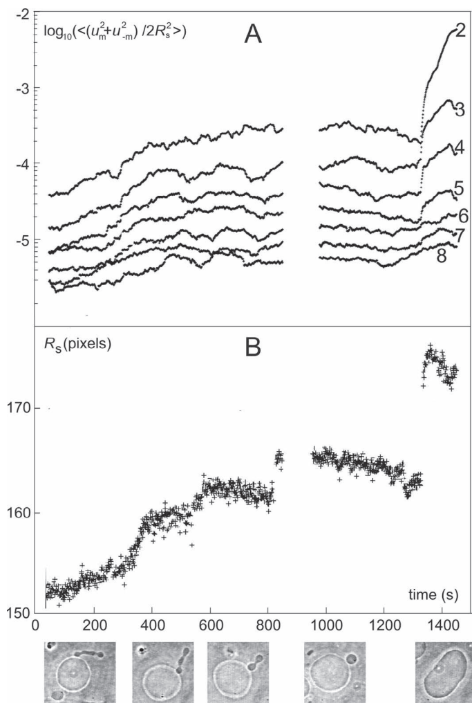
Figure 18.24 Time dependence of the average (moving averages over 100 points) square of the Fourier coefficients normalized by the square of the effective radius \langle (u_m + u_{-m})^2 / 2R_s^2 \rangle for m = 2 to 8 as indicated in panel A; the scale on the ordinate is logarithmic (A). Time dependence of the effective radius of the mother globule R_s along the same sequence where the shortened and undulating protrusion integrates with the globular part (B). Each point corresponds to one image. (Štukelj, 2013).
