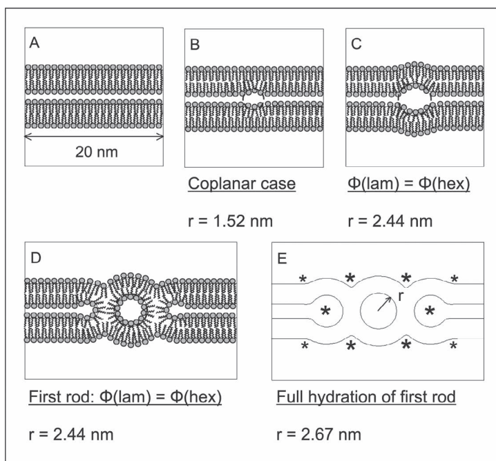
Figure 7.6 Intermediate steps in the formation of a cylinder between two bilayers. The structural schemes are based on structural data for POPE recorded at the transition temperature T = 74^\circ\text{C} (see Rappolt et al., 2003). Pivotal interfaces are outlined by full lines and for ease of interpretation lipid molecules are superimposed in the first four panels. (A) The fluid lamellar phase can be decomposed into a steric monolayer of thickness 2.27 nm and a free water layer of thickness 0.27 nm. (B) By spontaneous splay of lipid molecules a line defect may form, which is integrated in the stack of bilayers in a coplanar fashion. (C) If one sets the water concentration per lipid in the line defect, \Phi_{\text{hex}} , to be equal to the water concentration given in the fluid lamellar phase, \Phi_{\text{lam}} , then the radius of the pivotal plane increases from r = 1.52 nm to 2.44 nm. (D) This panel shows the formation of a first rod under the condition \Phi_{\text{lam}} = \Phi_{\text{hex}} . (E) Finally, full hydration of the first cylinder between two bilayers increases the pivotal plane radius to r = 2.67 nm. Loci for the formation of new cylinders are marked with stars (Perutková et al., 2009; Rappolt et al., 2008). Reprinted from Chemistry and Physics of Lipids , 154(1), Michael Rappolt, Aden Hodzic, Barbara Sartori, Michel Ollivon, Peter Laggner. Conformational and hydrational properties during the L_\beta - to L_\alpha - and L_\alpha - to H_{II} -phase transition in phosphatidylethanolamine, pp. 46–55, Copyright 2008, with permission from Elsevier.
