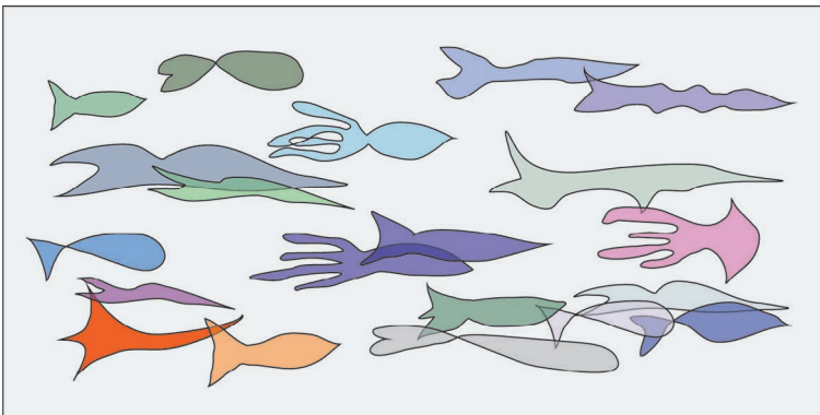
Figure 1.2 Schematic figure of a vector field without sources, sinks and vortices.
