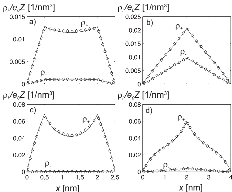
Figure 14.12 The volume charge density profile ( \rho_i(x) ) of divalent spherical nanoparticles ( l = 2 \text{ nm} , Z = 1 ) between two negatively charged surfaces calculated for two different values of charge parameter P and two different distances D : (a) P = -0.1 , D = 2.5 \text{ nm} ; (b) P = -0.1 , D = 4 \text{ nm} ; (c) P = -0.5 , D = 2.5 \text{ nm} ; (d) P = -0.5 , D = 4 \text{ nm} . Theoretical predictions of \rho_i(x) (lines) are compared to corresponding MC results (diamonds and circles). Reprinted with kind permission from Springer Science+Business Media: Perutková, Š., Frank, M., Bohinc, K., Bobojevič, K., Zelko, J., Rozman, B., Kralj-Iglič, V., and Iglič, A. (2010). Interaction between equally charged membrane surfaces mediated by positively and negatively charged nanoparticles. J. Membr. Biol. , 236, pp. 43–53.
